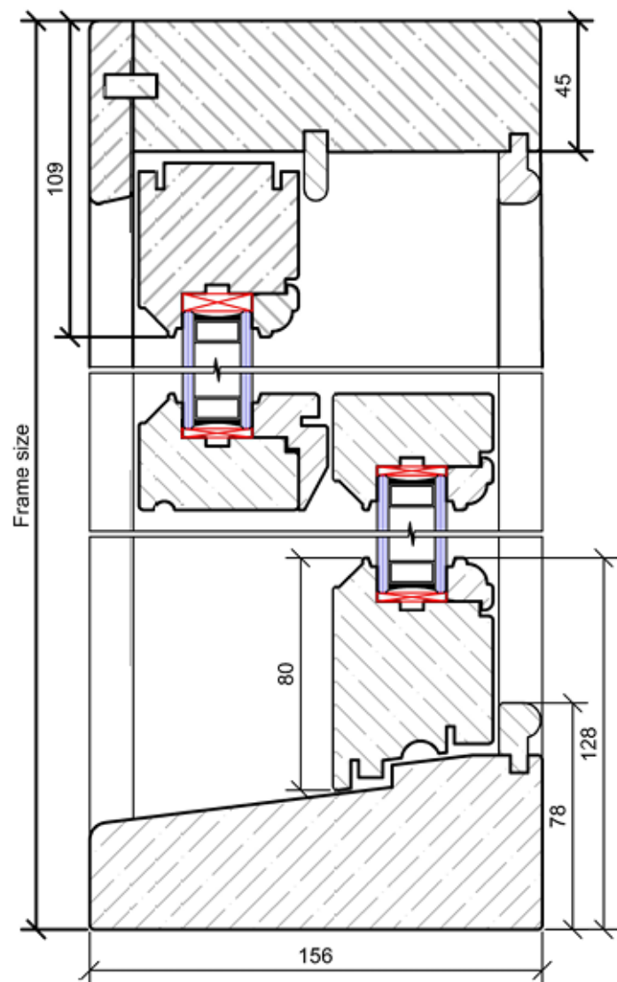
Vertical Section
