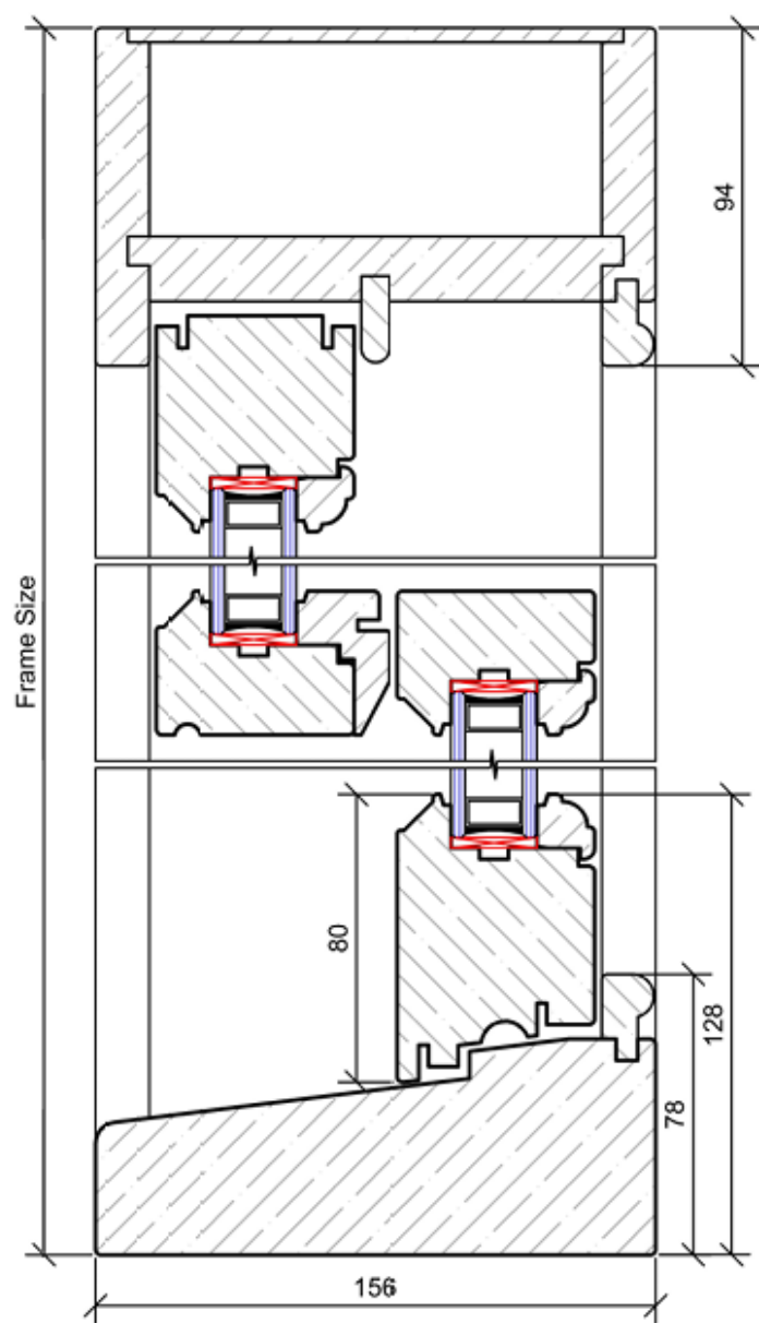
Vertical Section
